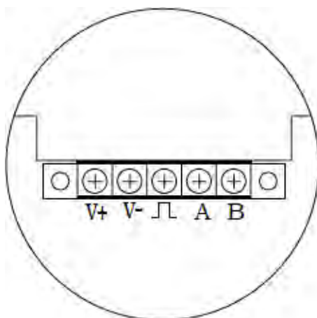
5-terminal Board
