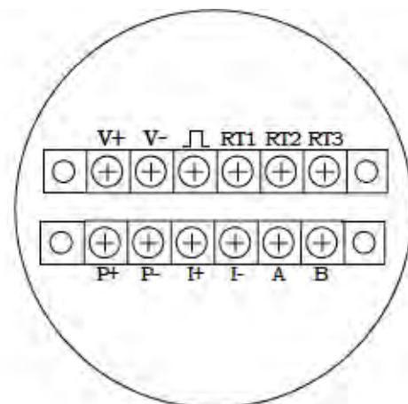
12-terminal Board
