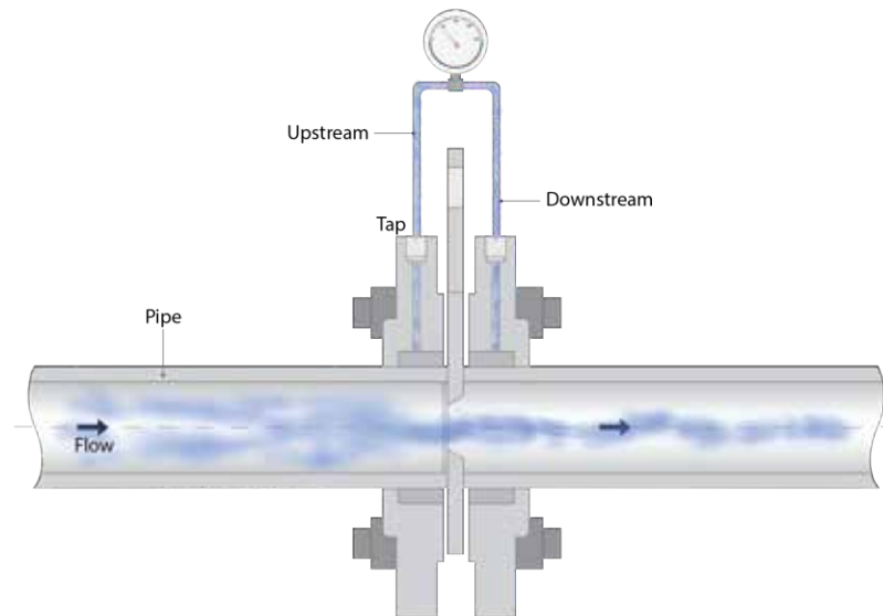
Fig.4. Differential Pressure Measurement
