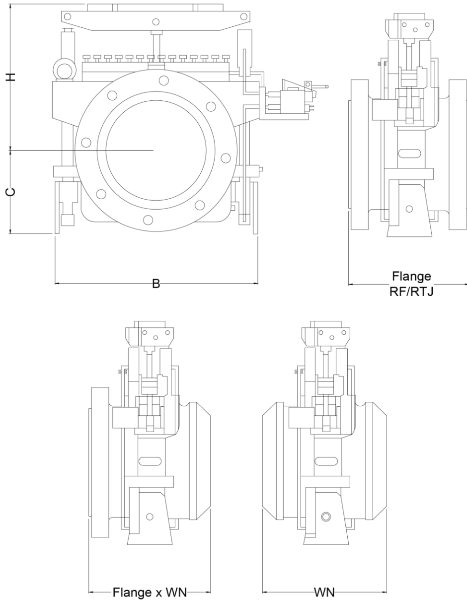
Fig.6. Dual Chamber Orifice Flowmeter
