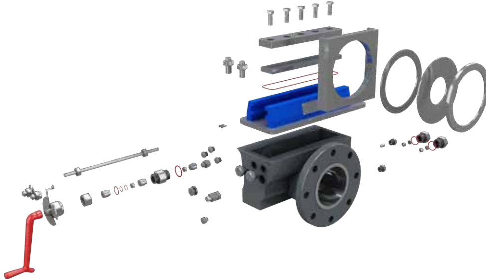
Fig. 8. Single exploded View
