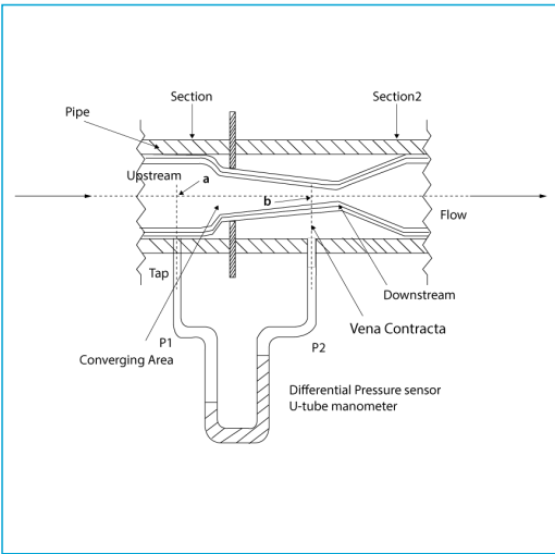
Fig 2. Measuring Principle
