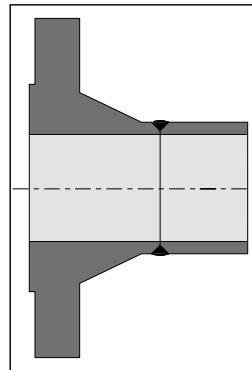
Fig 9: Welding Neck Flange
