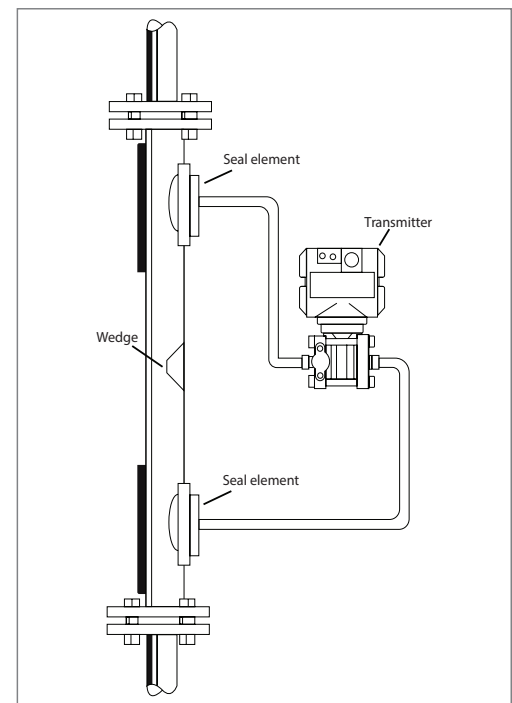
Fig 9: Vertical Installations
