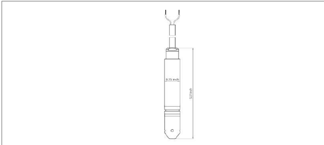
Fig.3 Dimension Drawing
