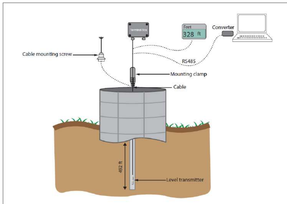
Fig.2. Mounting the transmitter
