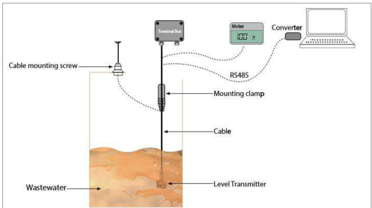
Fig.2. Mounting the transmitter
