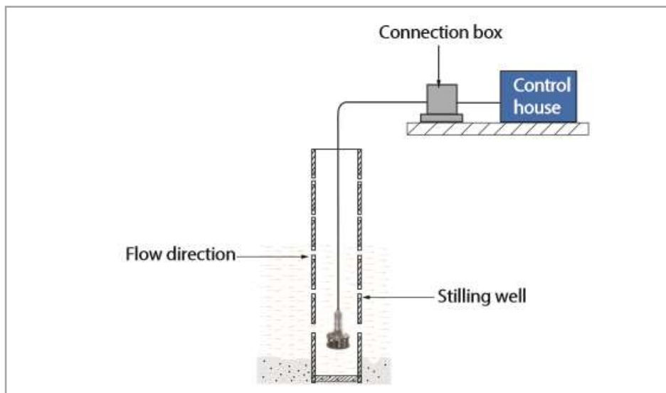
Fig.5. Installation in flowing liquid
