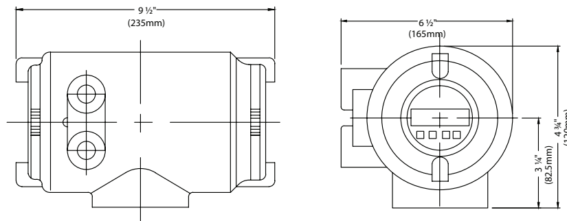
Direct Mount Transmitter
