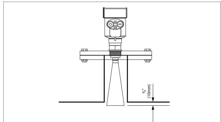
Fig 12: Installation with Height Requirement
